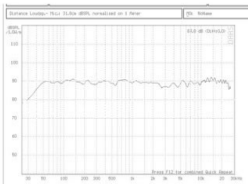
BD No 2 Frequency Response
